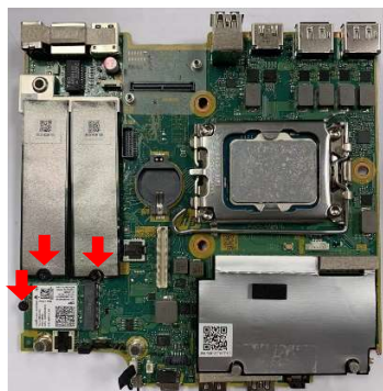
SSD PCB
