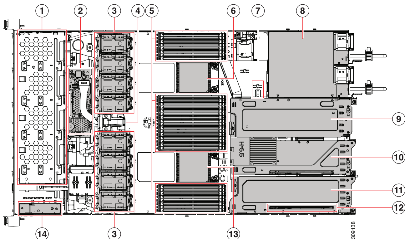
Figure 9 HX220C M6 All NVMe/All Flash/Hybrid Server Nodes With Top Cover Off (full-height, half-width PCIe cards)
