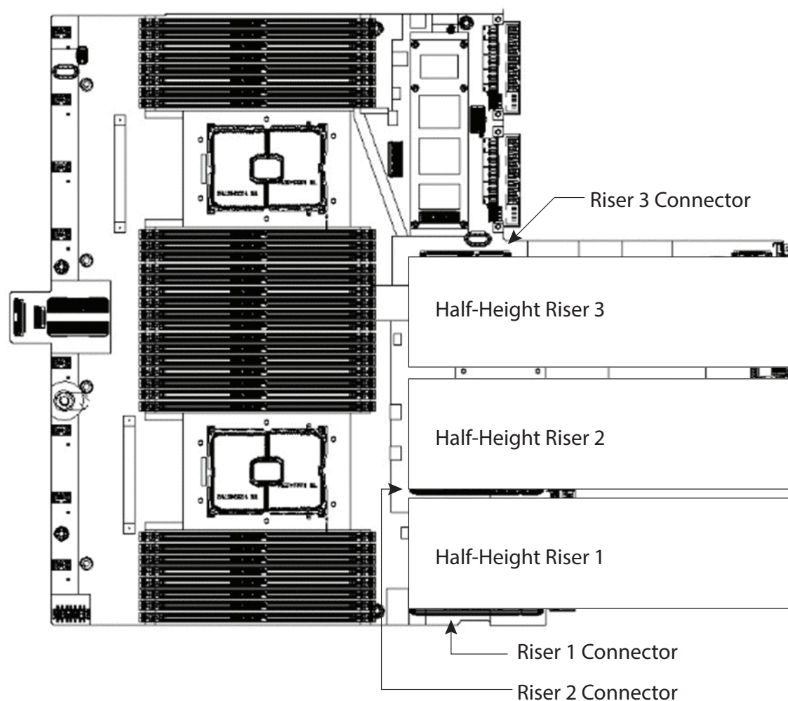
Figure 11 Cisco HyperFlex Express HX220C M6 All NVMe/All Flash/Hybrid Server Nodes with three half-height risers plugged in HX220M6 Motherboard
