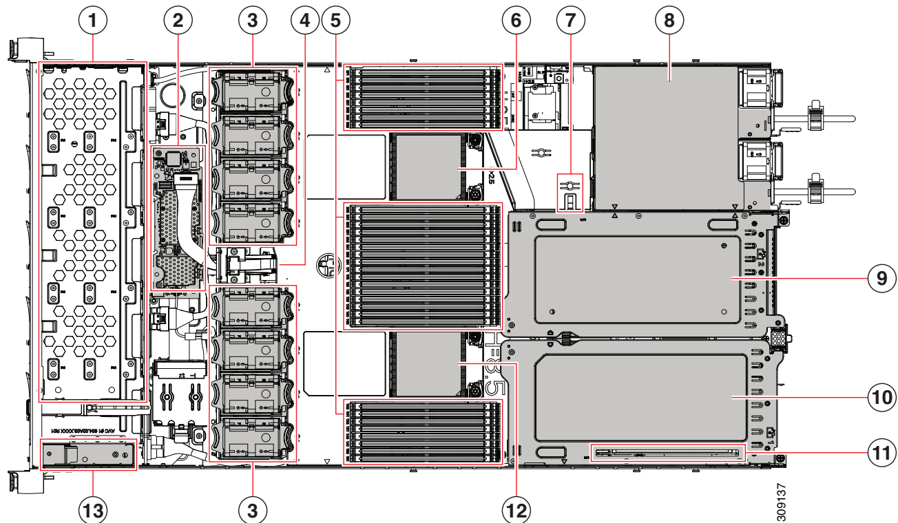
Figure 8 Cisco HyperFlex Express HX220C M6 All NVMe/All Flash/Hybrid Server Nodes With Top Cover Off (full-height, full-width PCIe cards)
