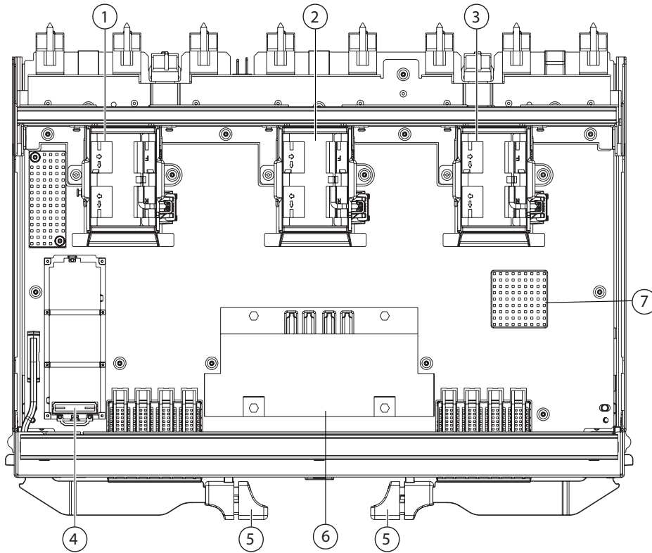
Figure 7 Cisco UCS 9108-25G IFM (top view)
