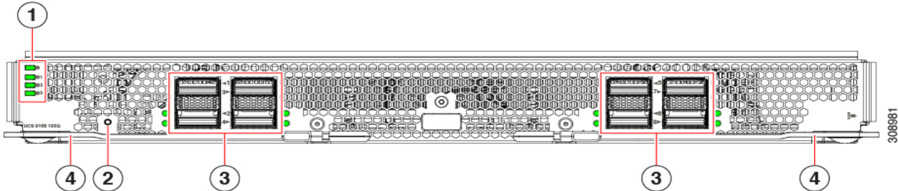
Figure 6 Cisco UCS 9108-100G IFM (front view)
