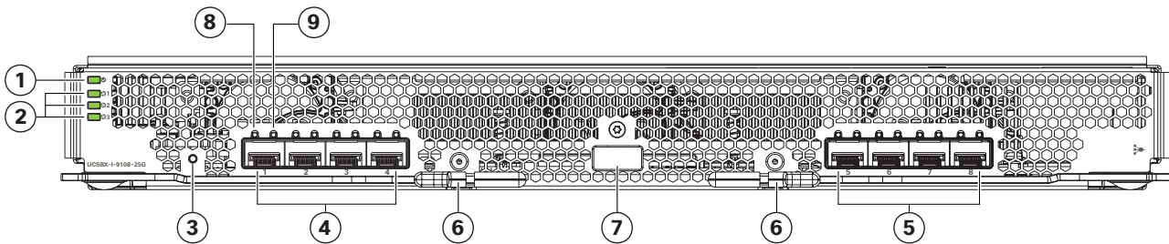
Figure 5 Cisco UCS 9108-25G IFM (front view)
