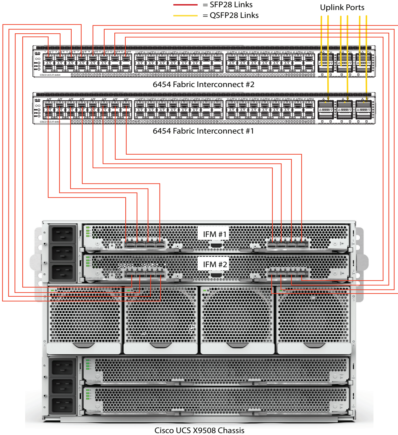
Figure 10 IFM to 6400 Series Fabric Interconnect Connectivity
