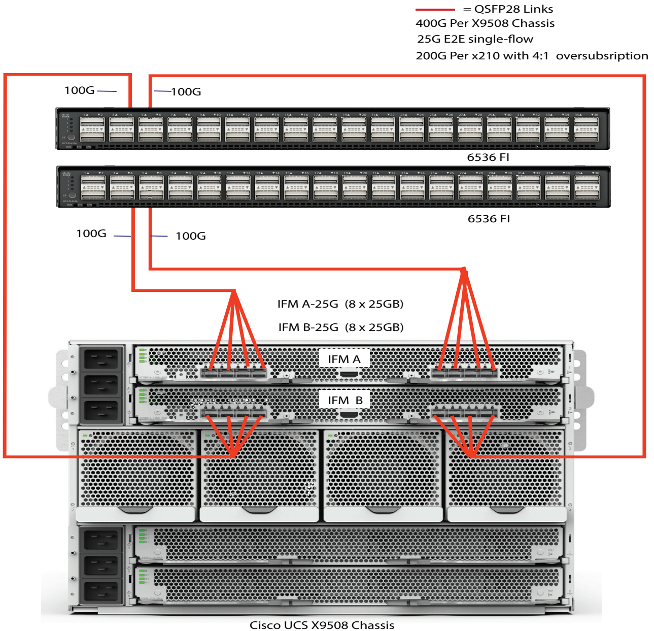
Figure 11 X9108-IFM-25G to 6536 Series Fabric Interconnects Connectivity
