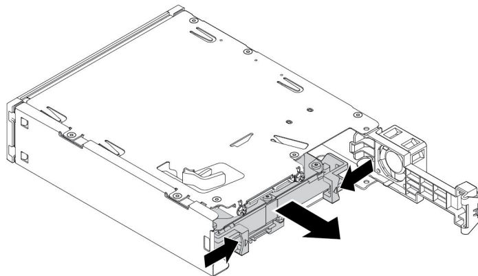
Figure 70. Removing the 3.5-inch internal storage drive from the rear
