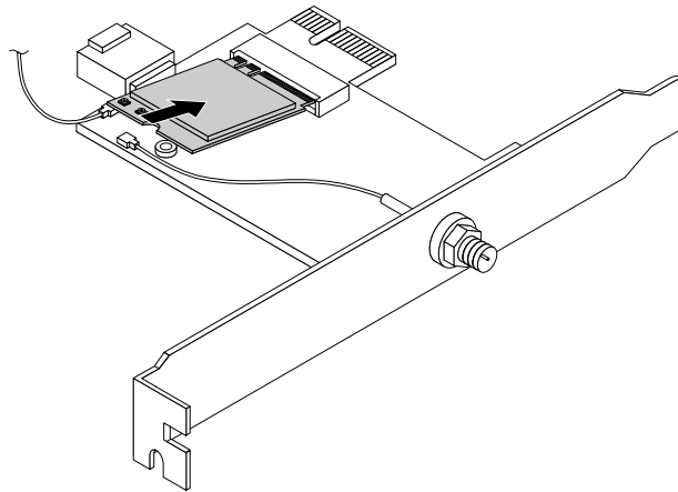
Figure 134. Installing the Wi-Fi card module
