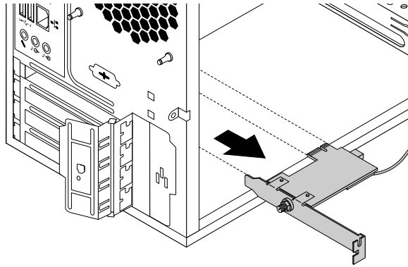
Figure 128. Removing the Wi-Fi adapter card
