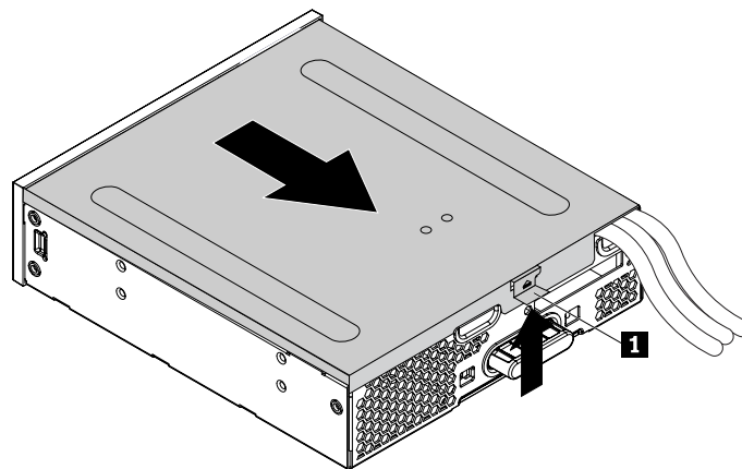
Figure 35. Removing the flex module cover
