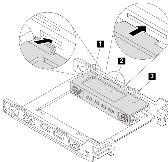
Figure 84. Inserting tabs 1 and 3 into the corresponding slots
