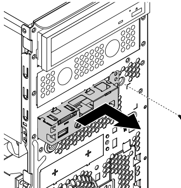
Figure 91. Removing the front audio and USB assembly
