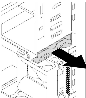
Figure 107. Removing the primary hard disk drive
