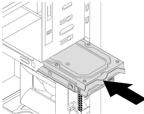
Figure 109. Installing the primary hard disk drive
