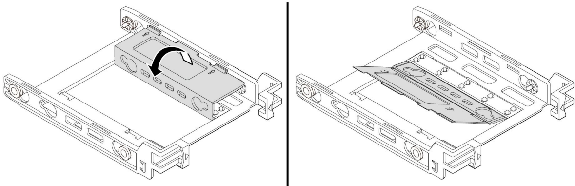
Figure 87. Unfolding the bracket
