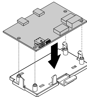
Figure 56. Installing the front Thunderbolt I/O adapter into the retaining bracket
