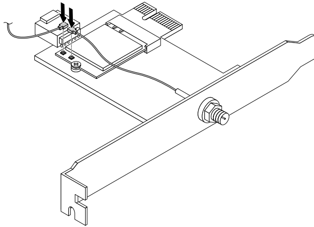
Figure 136. Installing the Wi-Fi antenna cables
