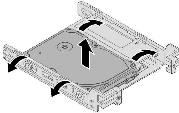
Figure 77. Flexing both sides of the bracket to remove the 2.5-inch internal storage drive
