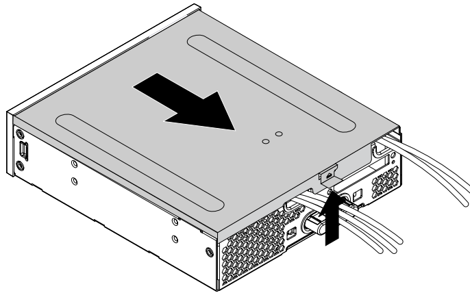
Figure 52. Removing the flex module cover
