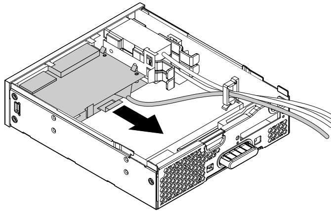
Figure 47. Removing the card reader from the flex module
