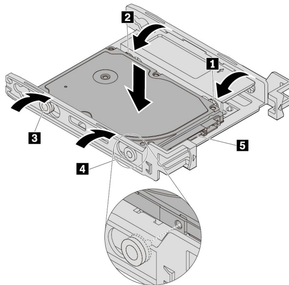
Figure 78. Installing the new 2.5-inch internal storage drive into the bracket
