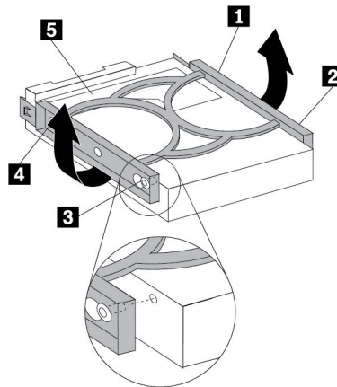
Figure 108. Installing the hard disk drive into the bracket
