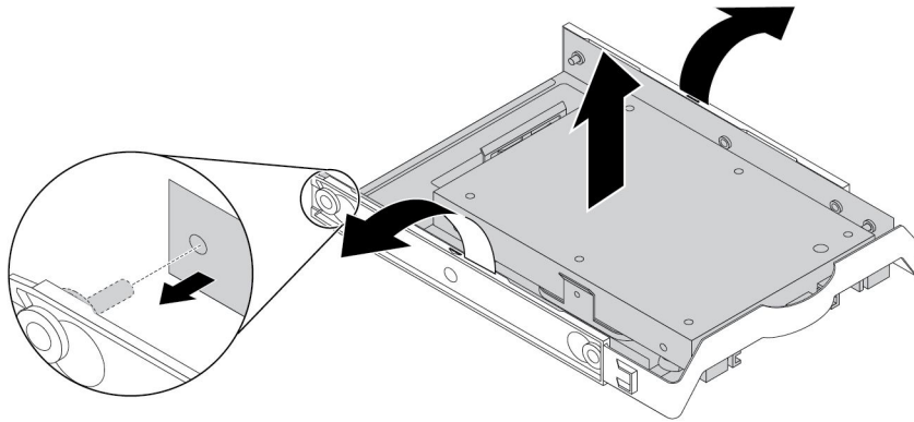
Figure 115. Removing the storage converter from the 3.5-inch storage drive bracket
