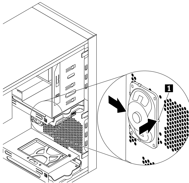
Figure 93. Removing the old internal speaker
