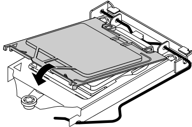
Figure 106. Installing the microprocessor socket cover
