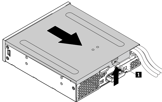
Figure 46. Removing the flex module cover
