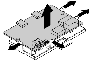
Figure 54. Removing the front Thunderbolt I/O adapter from the retaining bracket
