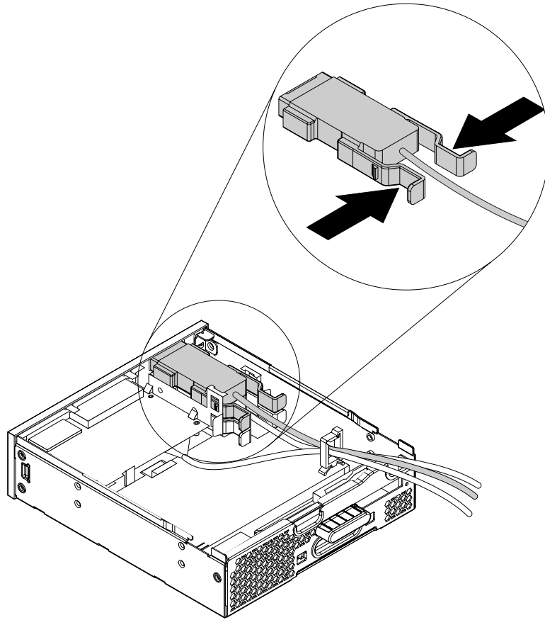
Figure 43. Removing the eSATA connector or IEEE 1394 connector from the flex module
