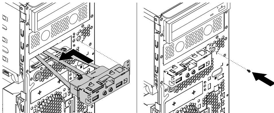
Figure 92. Installing the front audio and USB assembly
