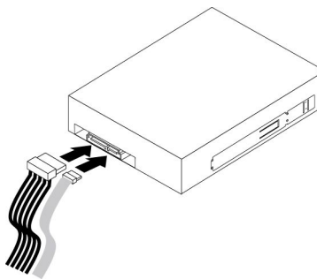
Figure 34. Connecting the cables to the rear of the new optical drive
