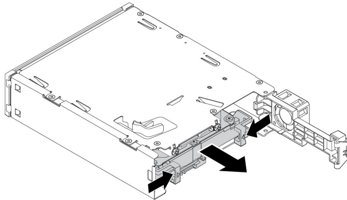
Figure 76. Removing the 2.5-inch internal storage drive from the rear
