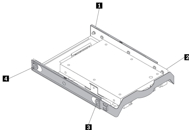
Figure 114. Installing the storage converter together with the solid-state drive into the storage drive bracket
