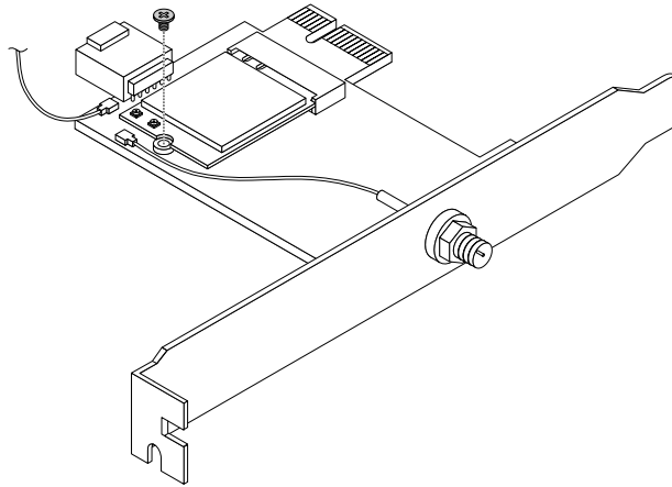
Figure 130. Removing the screw that secures the Wi-Fi card module
