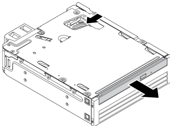
Figure 65. Removing the slim optical drive from the kit
