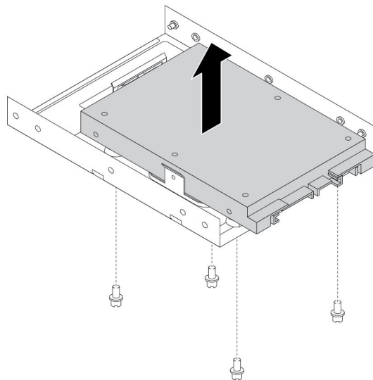
Figure 116. Removing the solid-state drive from the storage converter
