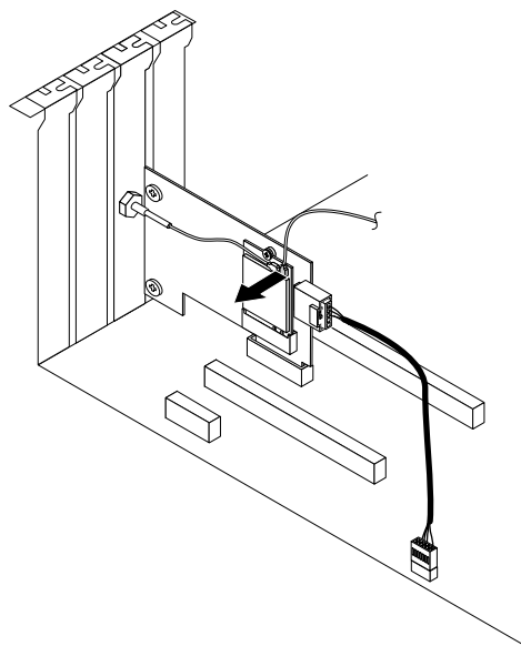
Figure 123. Disconnecting the front Wi-Fi antenna cable
