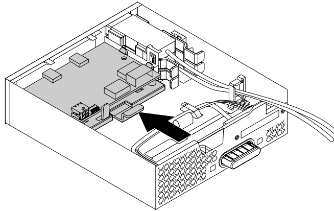
Figure 57. Installing the front Thunderbolt adapter and the retaining bracket into the flex module
