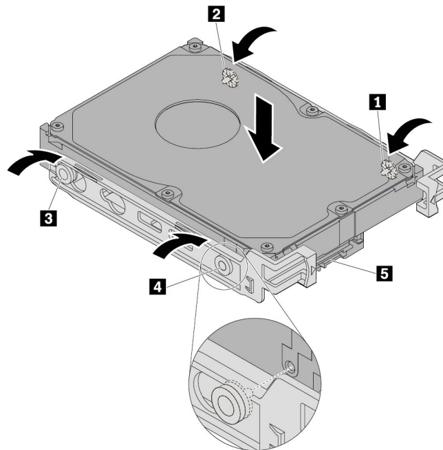
Figure 72. Installing the new 3.5-inch internal storage drive into the bracket
