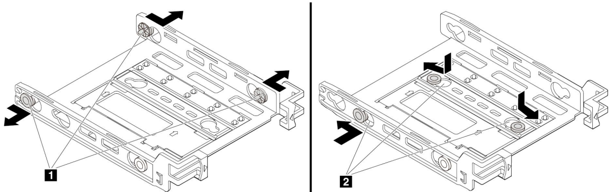
Figure 81. Removing three pins and installing them into new slots
