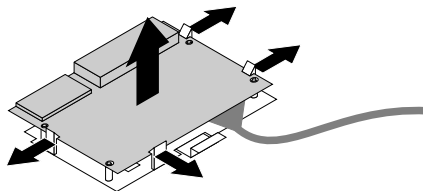
Figure 48. Removing the card reader from the card-reader retaining bracket
