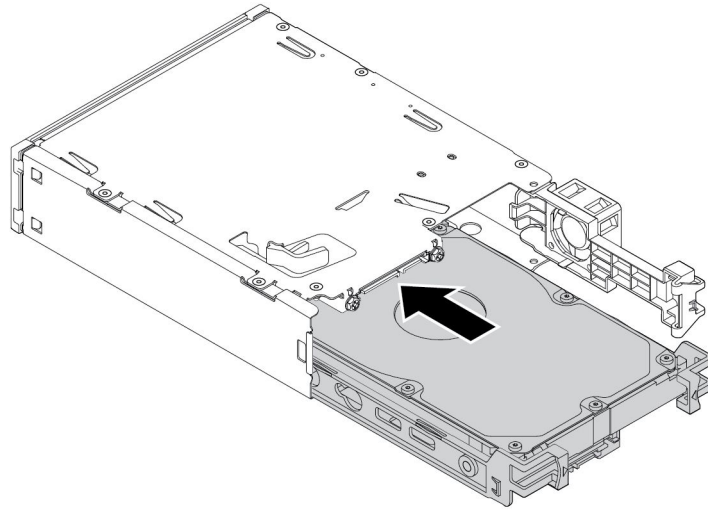
Figure 73. Sliding the new 3.5-inch internal storage drive into the kit
