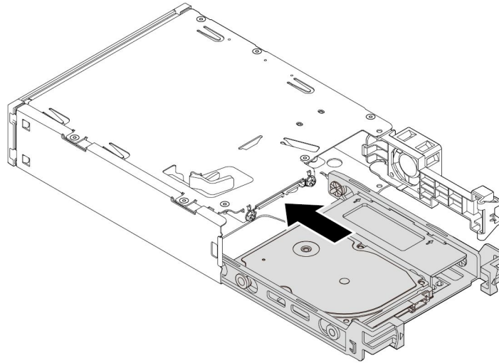
Figure 79. Sliding the new 2.5-inch internal storage drive into the kit
