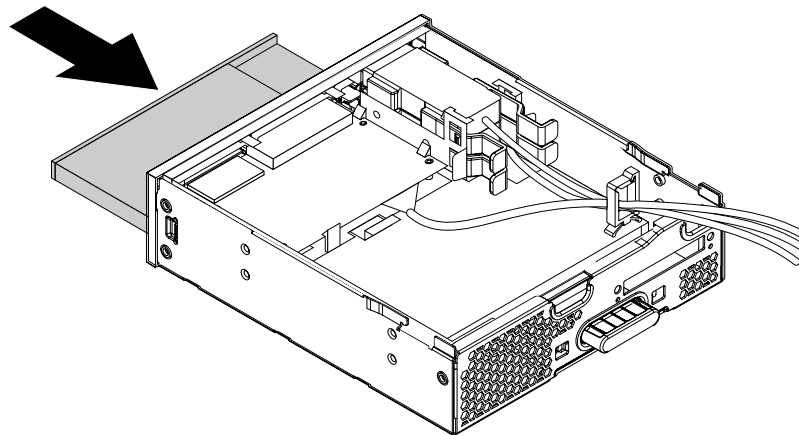
Figure 40. Installing the slim optical drive in the flex module
