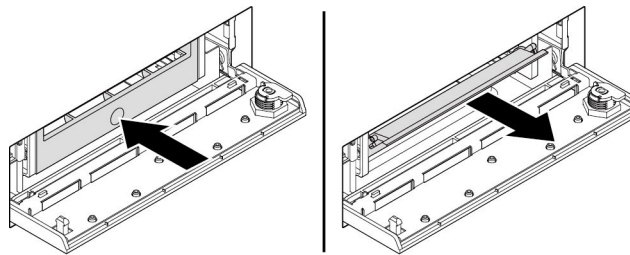
Figure 61. Removing the hard disk drive from the front-access storage enclosure
