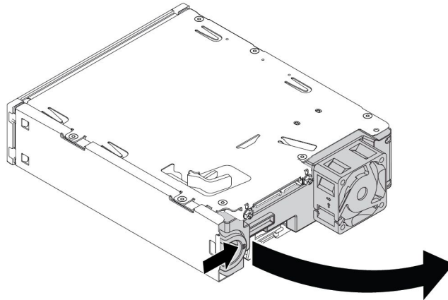
Figure 75. Opening the kit from the rear
