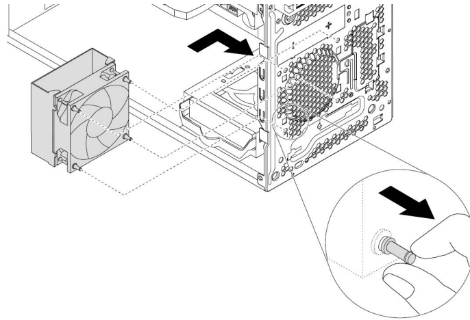
Figure 120. Installing the front fan assembly
