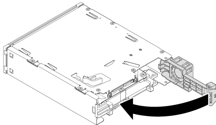
Figure 80. Pivoting the rear cover inward
