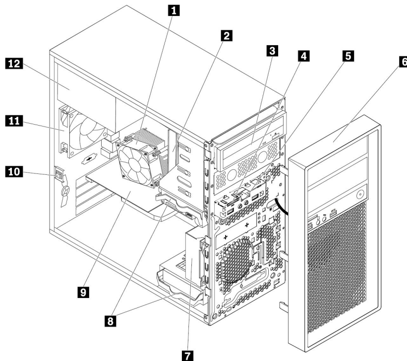
Figure 3. Computer components
