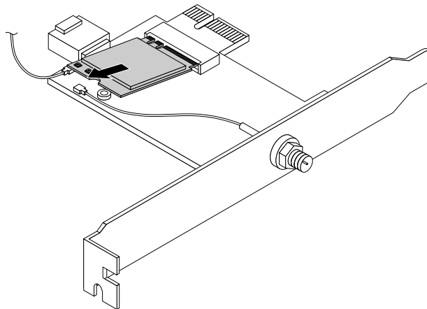
Figure 131. Removing the Wi-Fi card module
