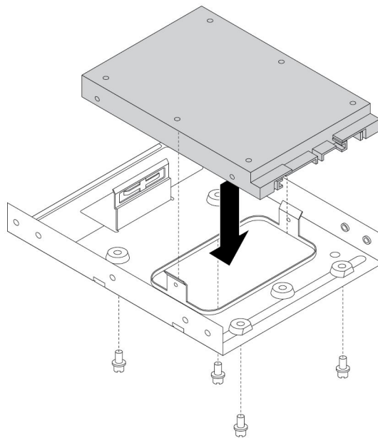
Figure 117. Installing the new solid-state drive into the storage converter
