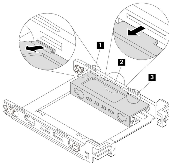
Figure 86. Releasing tabs 1 , 2 , and 3 from the corresponding slots
