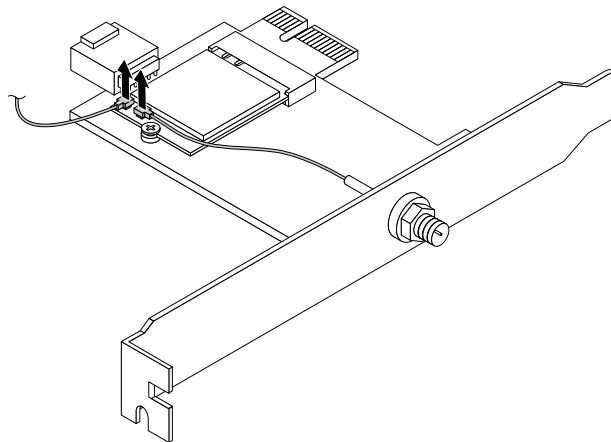
Figure 129. Disconnecting the Wi-Fi antenna cables
