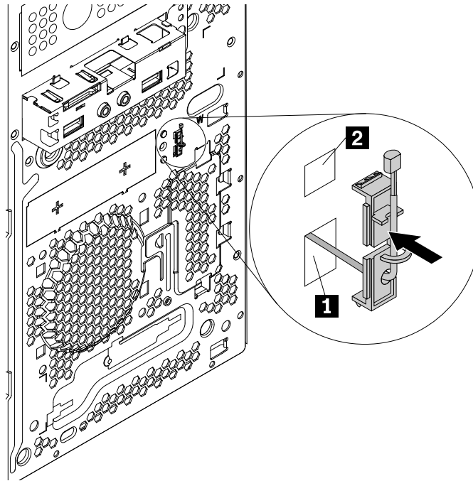
Figure 96. Installing the thermal sensor
