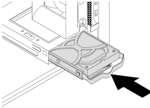
Figure 112. Installing the secondary hard disk drive
