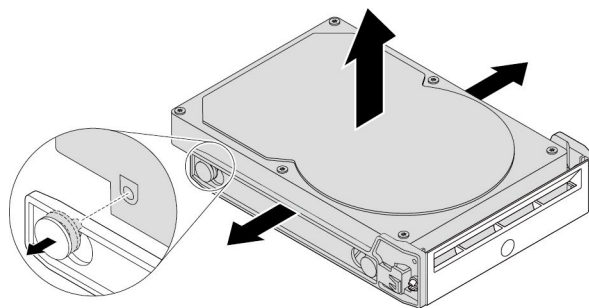
Figure 62. Removing the hard disk drive from the bracket
