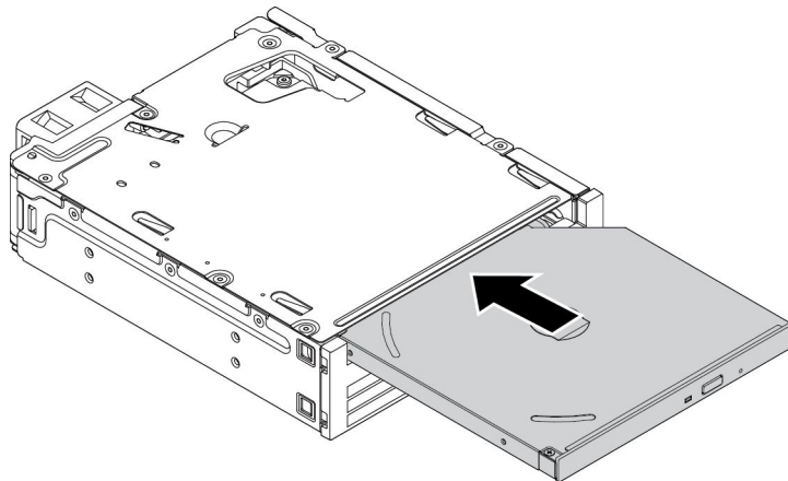
Figure 68. Installing the slim optical drive into the kit
