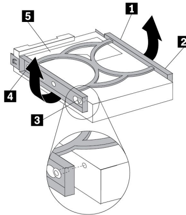
Figure 111. Installing the hard disk drive into the bracket
