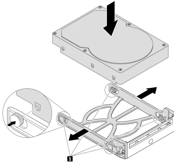
Figure 63. Installing the hard disk drive into the bracket
