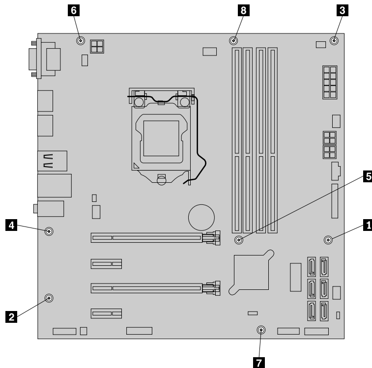
Figure 104. Removing the eight screws that secure the system board
