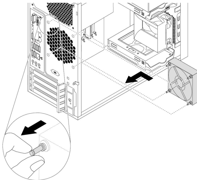
Figure 122. Installing the rear fan assembly
