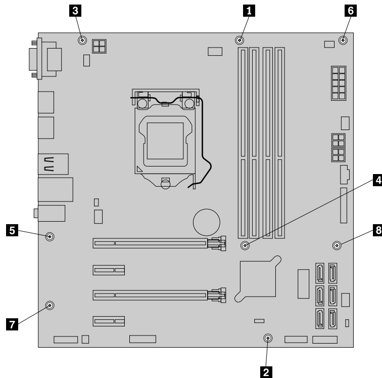
Figure 105. Installing the eight screws to secure the system board
