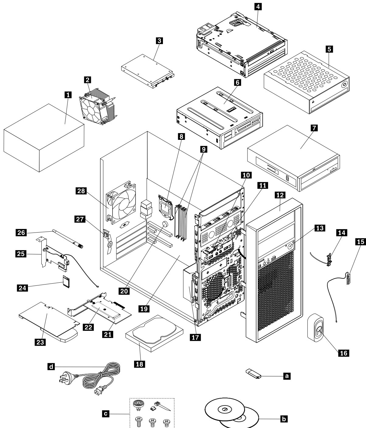
Figure 4. Major FRUs and CRUs
