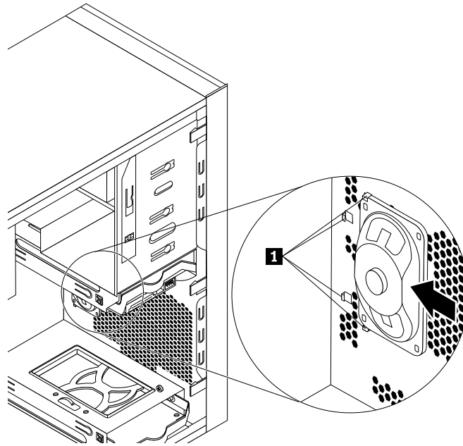
Figure 94. Installing the internal speaker
