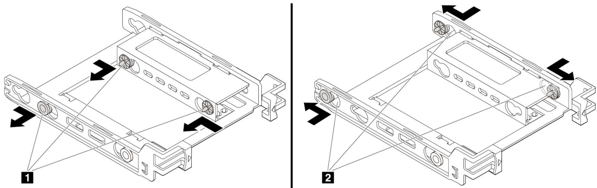
Figure 85. Removing three pins 1 and installing them into slots 2
