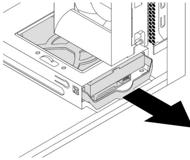
Figure 110. Removing the secondary hard disk drive
