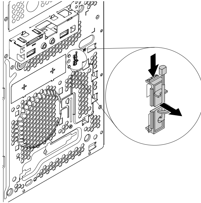
Figure 95. Removing the thermal sensor
