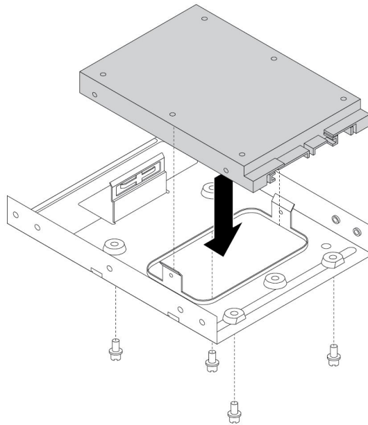
Figure 113. Installing the solid-state drive into the storage converter
