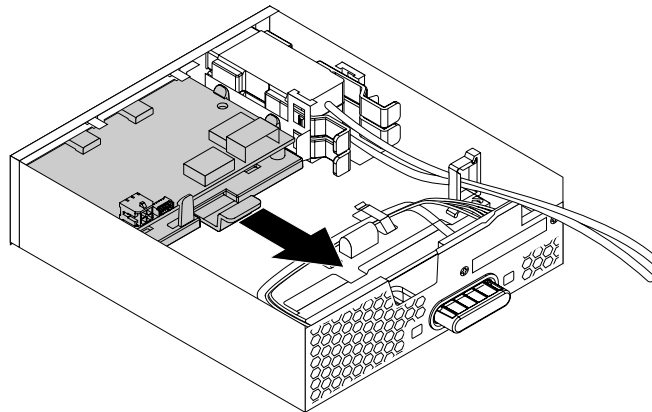
Figure 53. Removing the front Thunderbolt adapter and the retaining bracket out of the flex module
