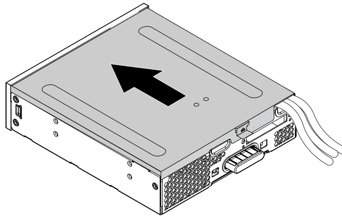
Figure 51. Reinstalling the flex module cover
