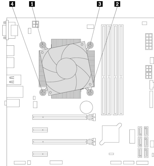
Figure 100. Removing the heat sink and fan assembly
