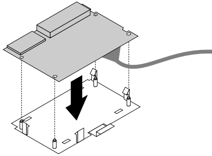
Figure 49. Installing the card reader into the card-reader retaining bracket
