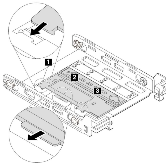
Figure 88. Inserting tabs 1 and 3 into the corresponding slots
