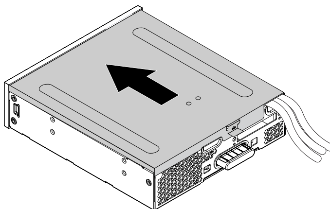
Figure 45. Reinstalling the flex module cover
