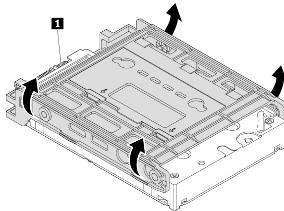
Figure 71. Flexing both sides of the bracket to remove the 3.5-inch internal storage drive
