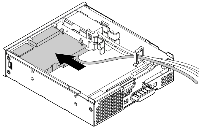
Figure 50. Installing the card reader in the flex module
