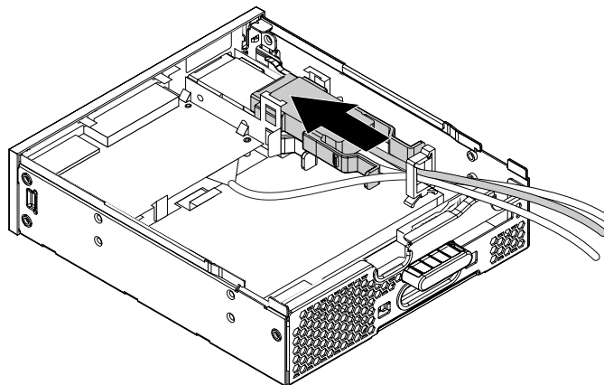
Figure 44. Installing the eSATA connector or IEEE 1394 connector in the flex module
