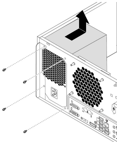
Figure 99. Removing the screws for the power supply assembly
