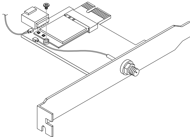
Figure 135. Installing a screw to secure the Wi-Fi card module
