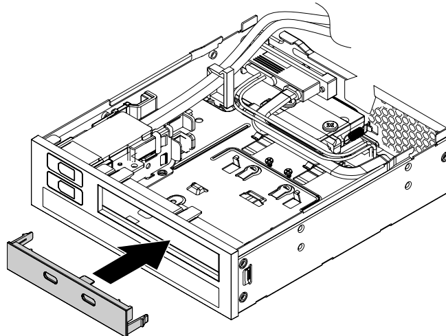
Figure 55. Installing the bezel to the flex module
