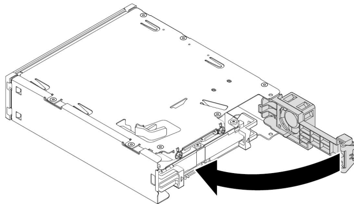
Figure 74. Pivoting the rear cover inward
