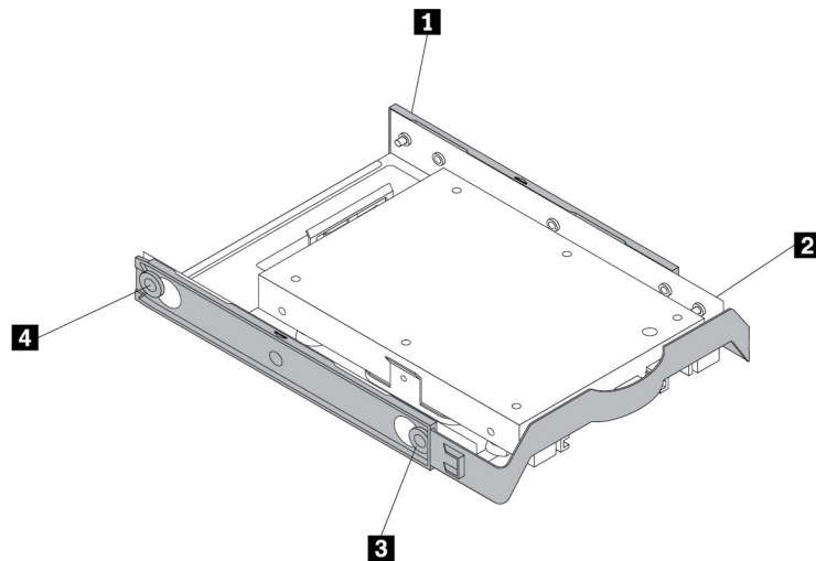
Figure 118. Installing the storage converter with the new solid-state drive into the storage drive bracket
