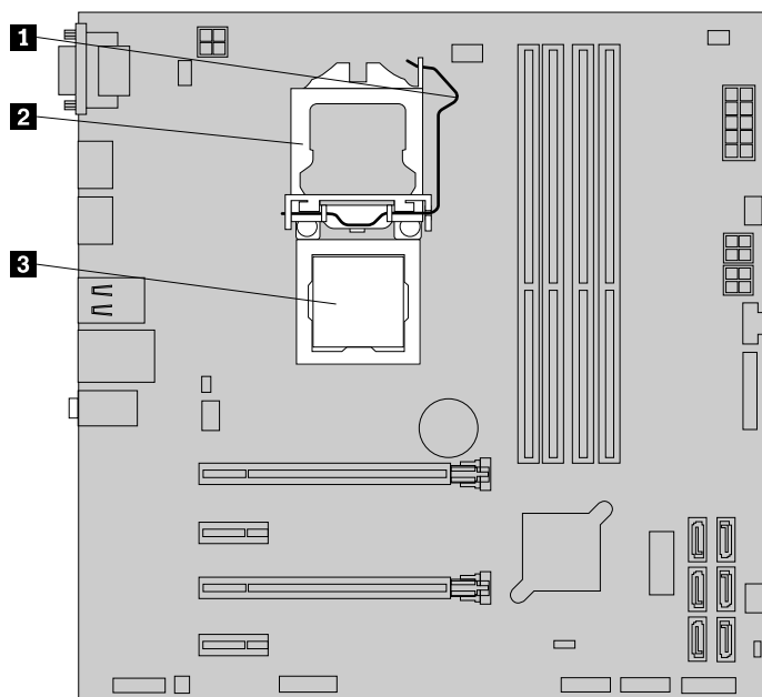
Figure 101. Accessing the microprocessor
