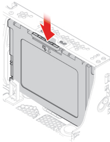
Figure 23. Removing the primary storage drive bracket
