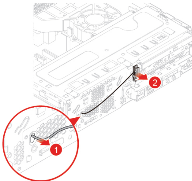
Figure 63. Removing the front Wi-Fi antenna
