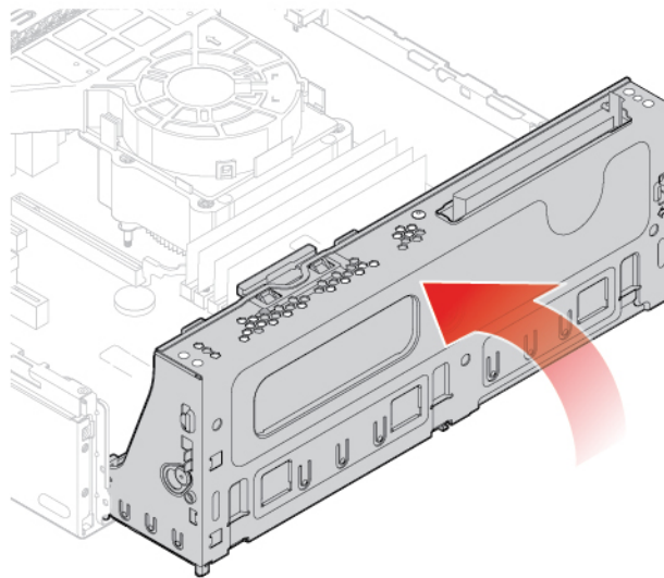
Figure 51. Pivoting the drive bay assembly downward
