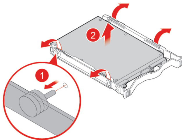
Figure 31. Removing the 2.5-inch secondary storage drive
